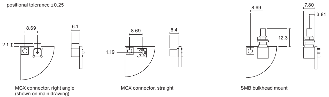
Figure 9-1: Jupiter 21 mechanical drawing
