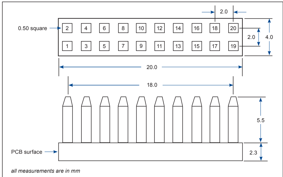
Figure 5-1: The 20-pin interface connector (J1)
